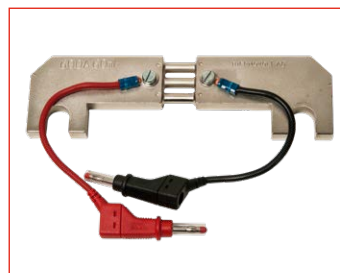
Calibration shunt, 600 A/60 mV (BB-90020)
