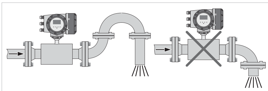
Figure 3-7: Open discharge
