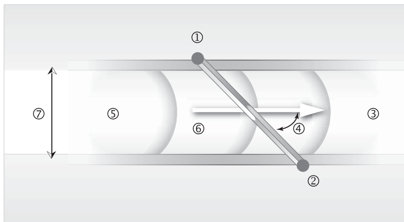
Figure 1-1: Measuring principle
