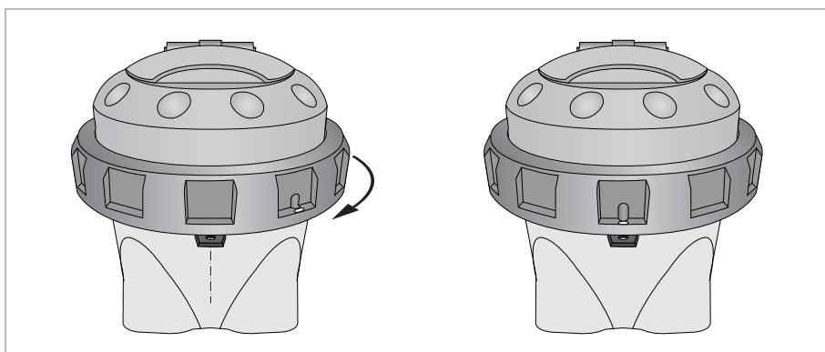
Figure 3-16: Closing of IP68 housing
