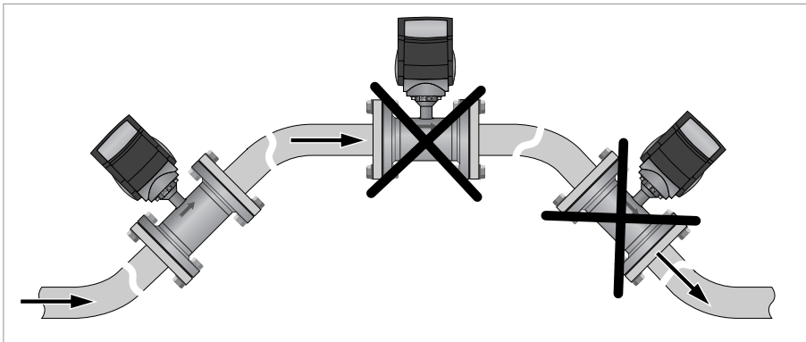
Figure 3-6: Installation in bending pipes
