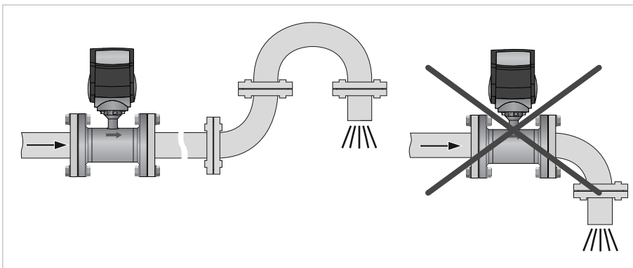
Figure 3-7: Installation in front of an open discharge
