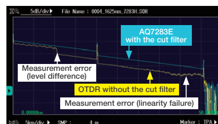
Trace examples of live communications lines
