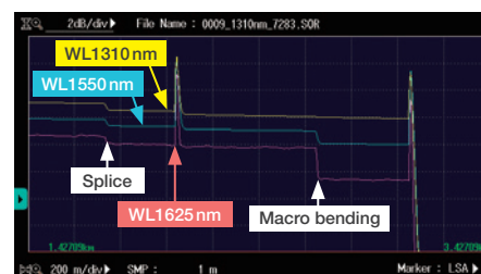
Trace examples with macro bending
