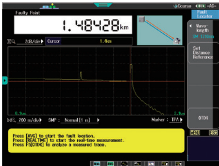
Example of detecting a breaking point 1.48 km away
