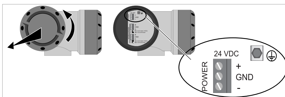
Figure 4-6: Location of power connector
