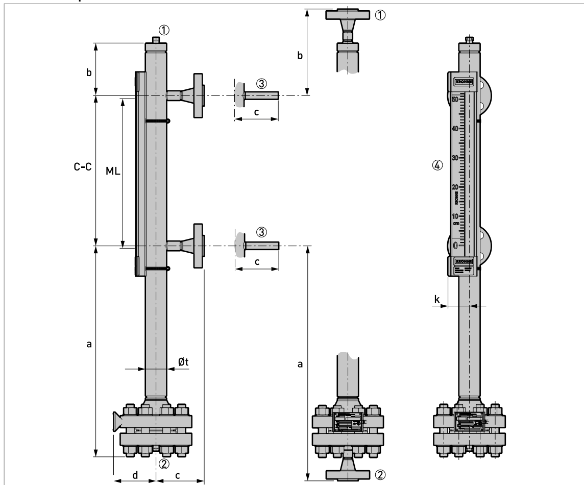
Figure 8-14: BM26A-7000 PN250 / Class 1500: side - side process connections
