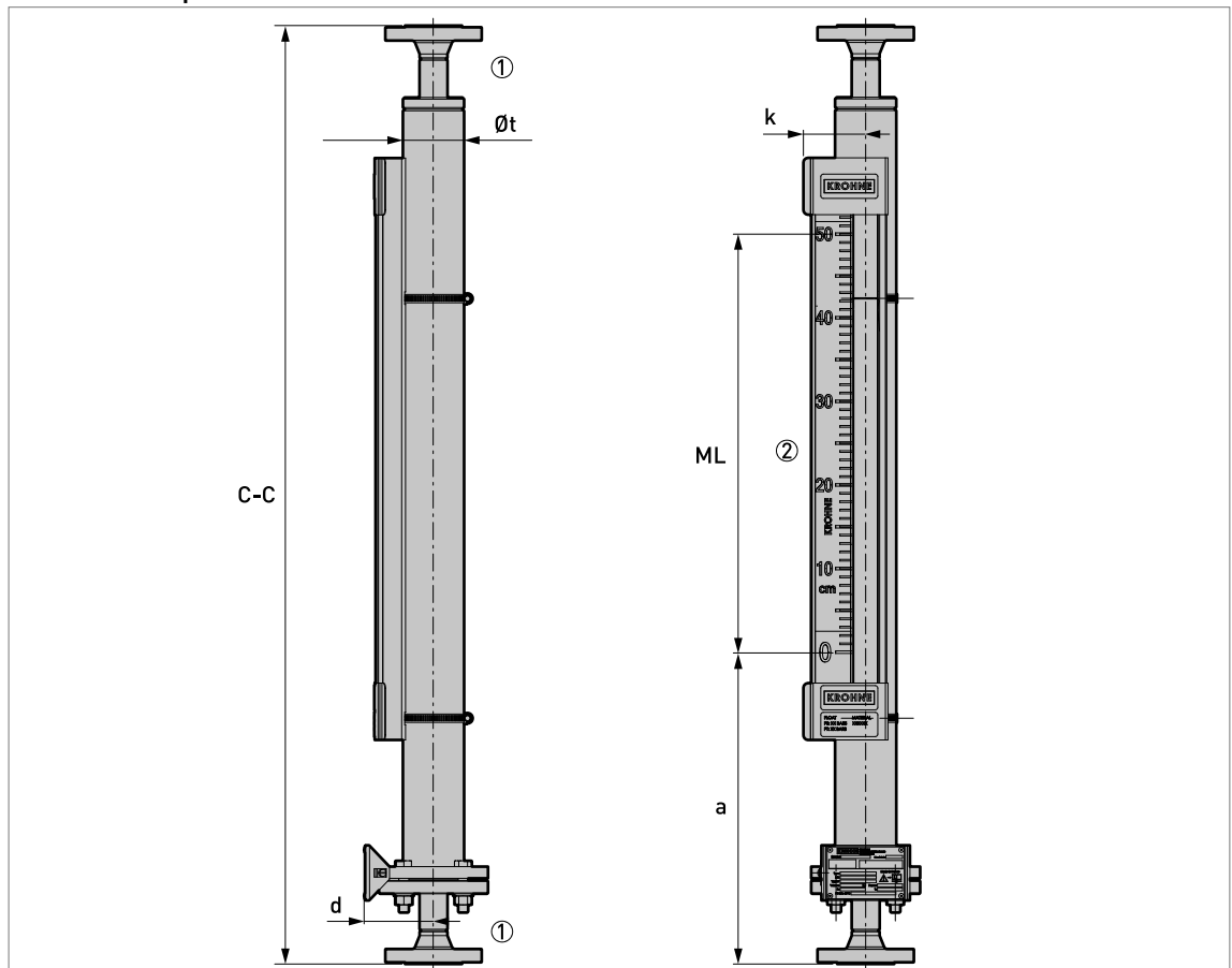
Figure 8-7: BM26A-7000 PN40 / Class 300: axial - axial process connections
