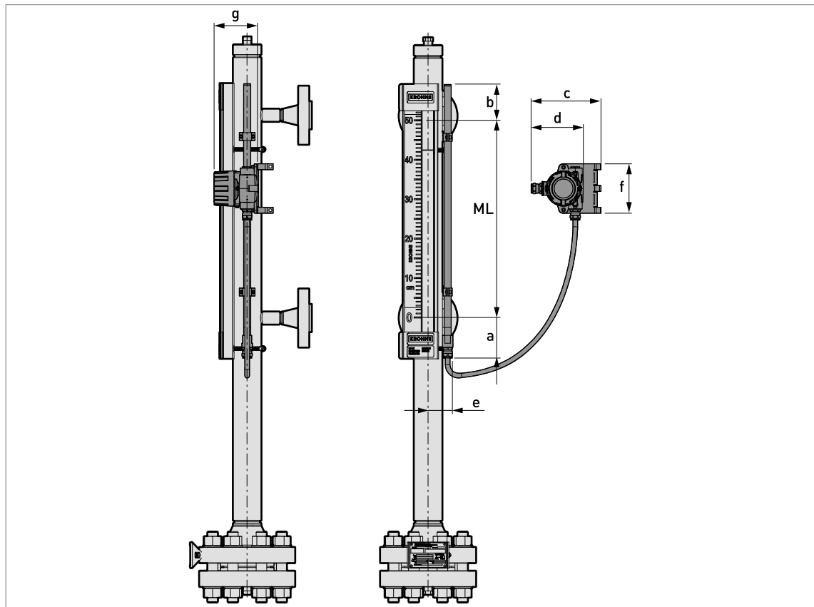
Figure 8-24: LT40 F reed-chain level transmitter - remote version
