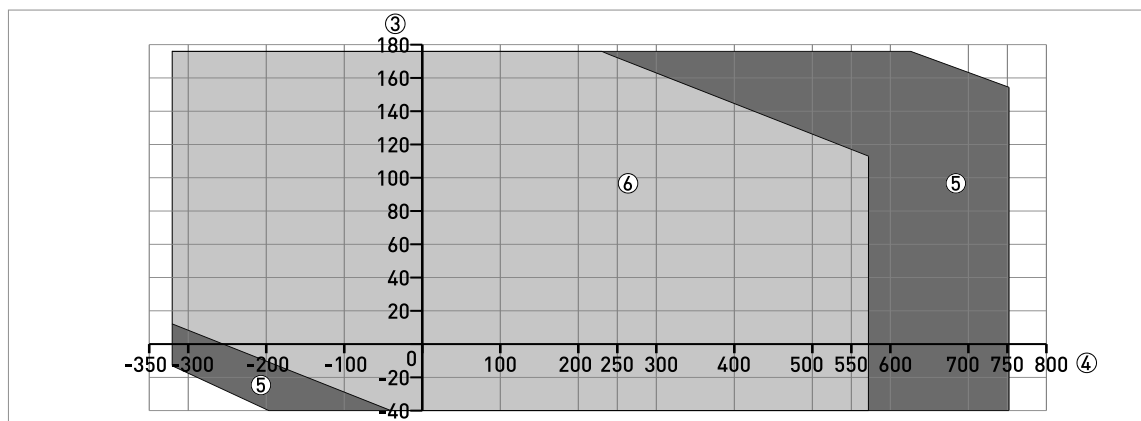
Figure 8-33: Ambient temperature / process temperature, in °F - with a thermal insulation option and without the LCD indicator module
