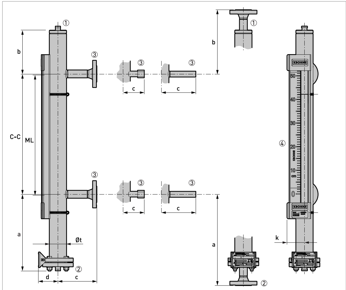
Figure 8-2: BM26A-6000: side - side process connections
