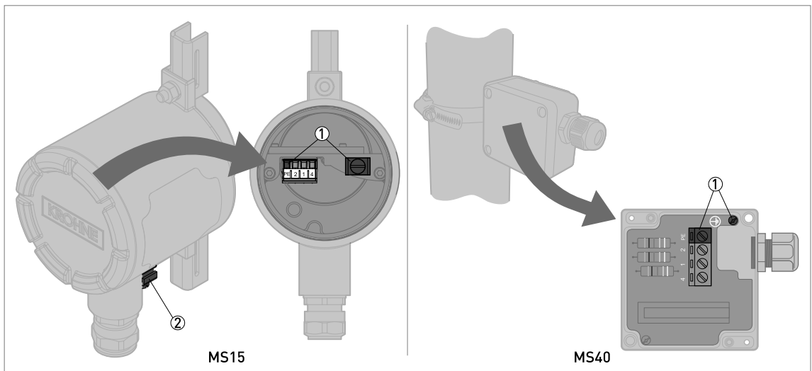
Figure 4-6: Limit switch - location of grounding terminals
