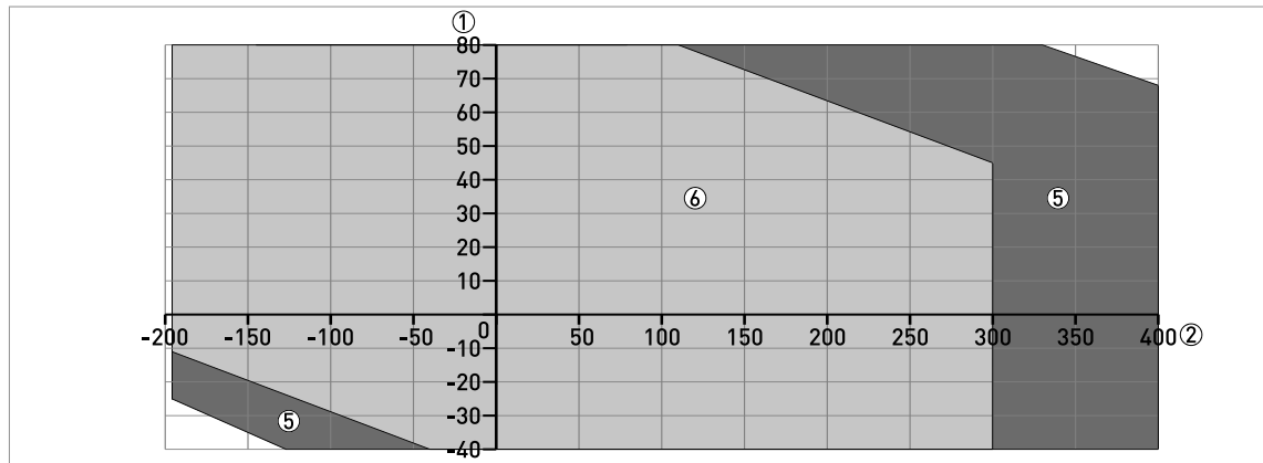
Figure 8-32: Ambient temperature / process temperature, in °C - with a thermal insulation option and without the LCD indicator module
