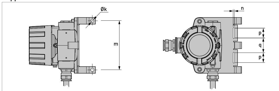
Figure 8-25: Support for the LT40 F reed-chain level transmitter
