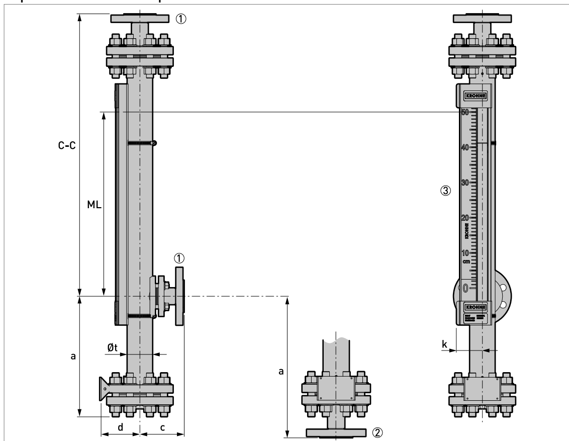
Figure 8-22: BM26A-7000 PN40 / Class 300 (PTFE-lined): top axial - bottom side process connections
