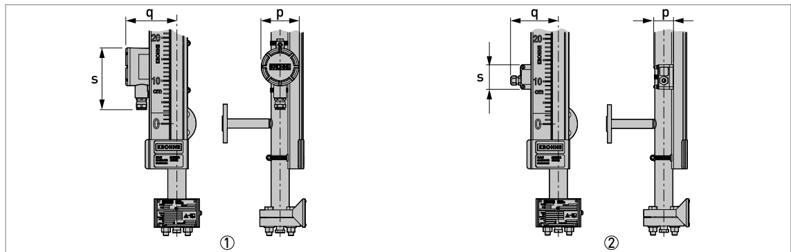
Figure 8-26: MS15-series and MS40-series limit switches
