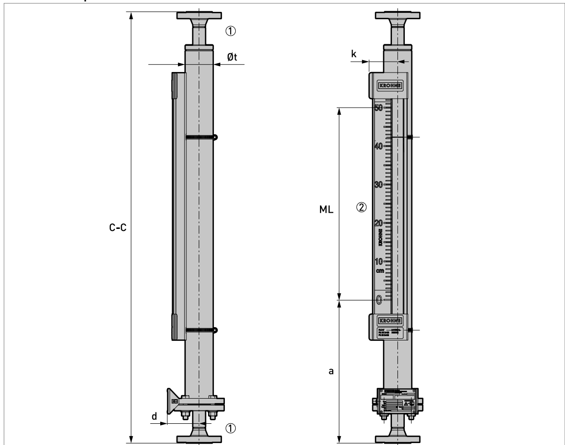
Figure 8-3: BM26A-6000: axial - axial process connections
