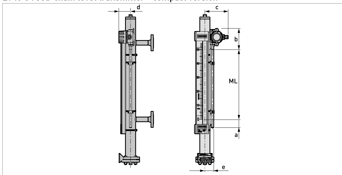
Figure 8-23: LT40 C reed-chain level transmitter - compact version
