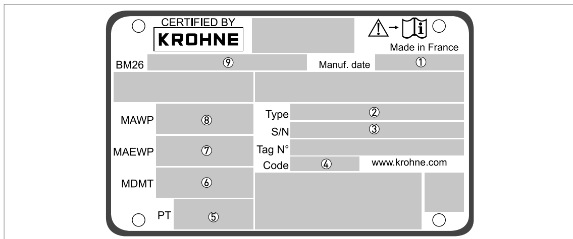
Figure 2-4: Measuring chamber nameplate [ASME B31.3 construction code]
