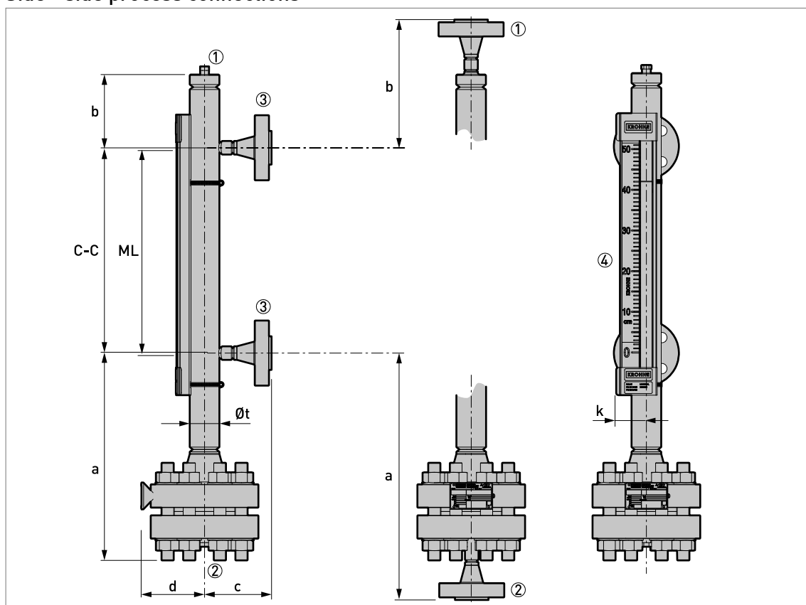
Figure 8-18: BM26A-7000 PN400 / Class 2500: side - side process connections
