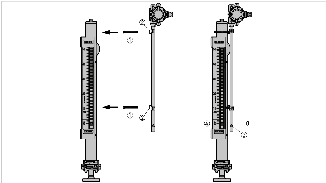
Figure 3-7: LT40: installation of the device on the measuring chamber
