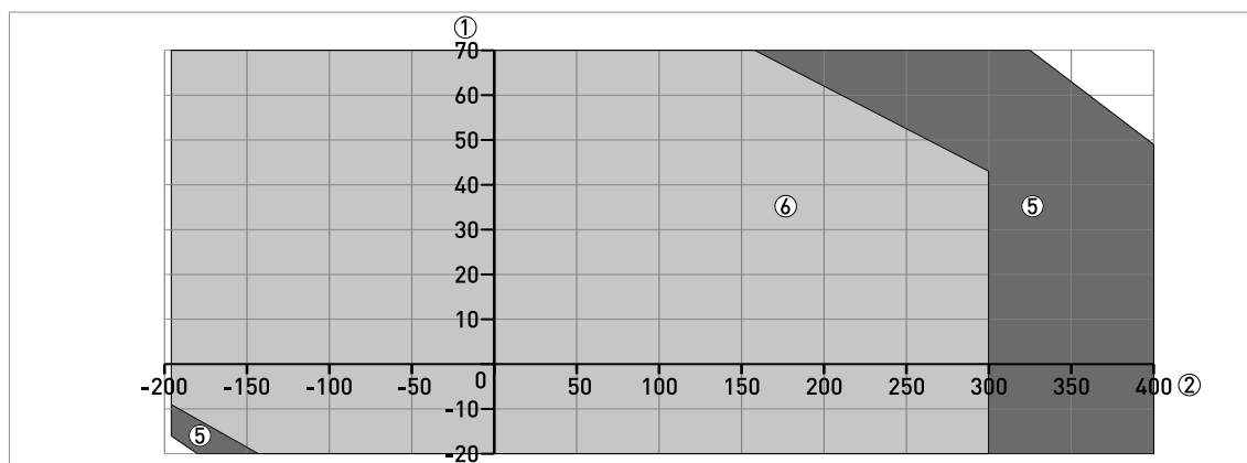
Figure 8-30: Ambient temperature / process temperature, in °C - without a thermal insulation option and with the LCD indicator module
