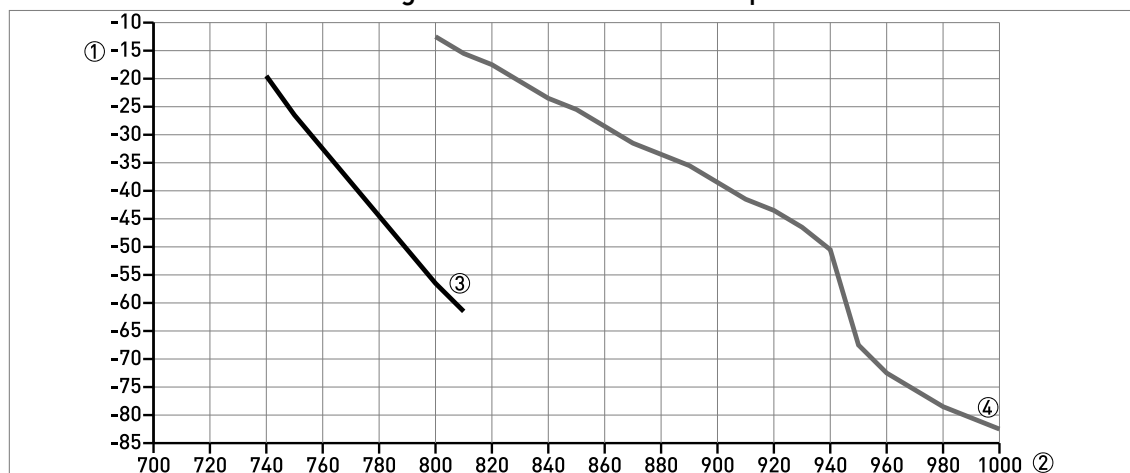
Figure 9-15: BM26A-7000 PN400: Float magnet offset in relation to liquid level in mm
