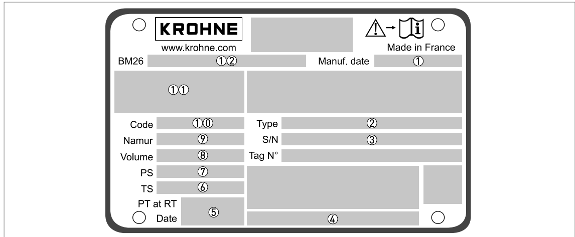
Figure 2-3: Measuring chamber nameplate (PED, PE(S)R and EN 13445 construction codes)
