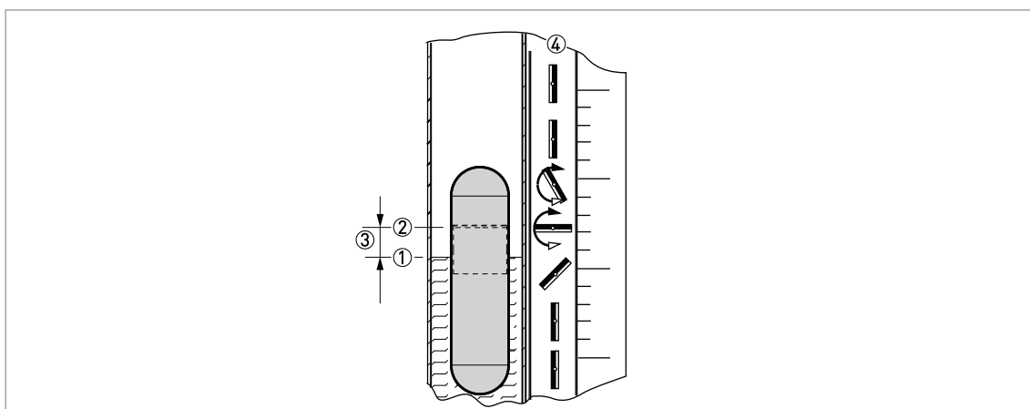
Figure 8-1: Offset between liquid level and the float magnet (liquid level offset)
