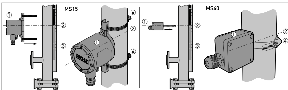
Figure 3-10: How to attach the limit switch to the measuring chamber
