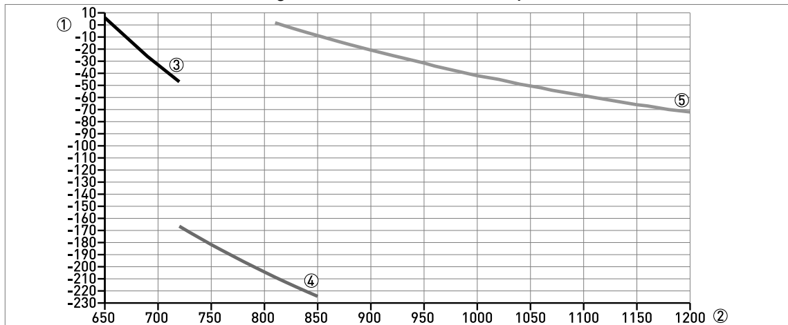
Figure 9-13: BM26A-7000 PN250: Float magnet offset in relation to liquid level in mm
