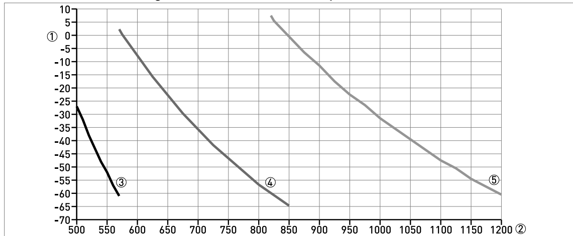
Figure 9-5: BM26A-6000: Float magnet offset in relation to liquid level in mm
