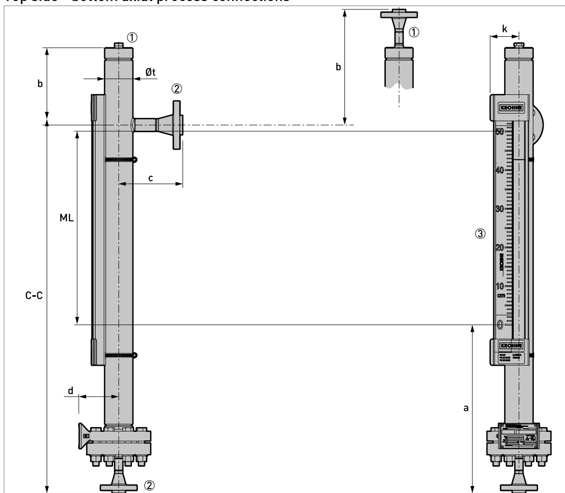
Figure 8-12: BM26A-7000 PN100 / Class 600: top side - bottom axial process connections
