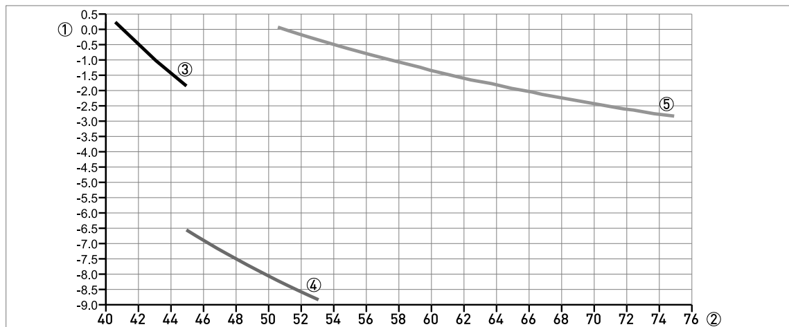
Figure 9-14: BM26A-7000 PN250: Float magnet offset in relation to liquid level in inches
