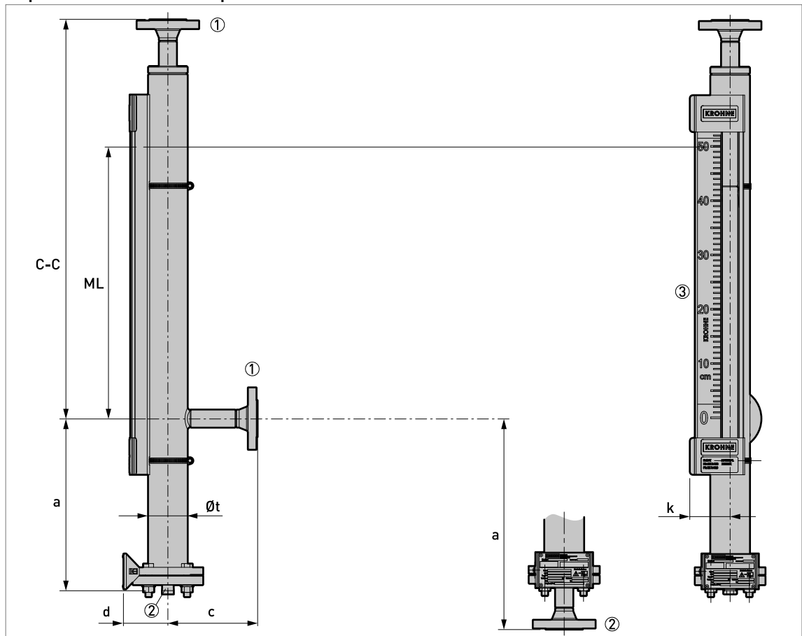
Figure 8-9: BM26A-7000 PN40 / Class 300: top axial - bottom side process connections
