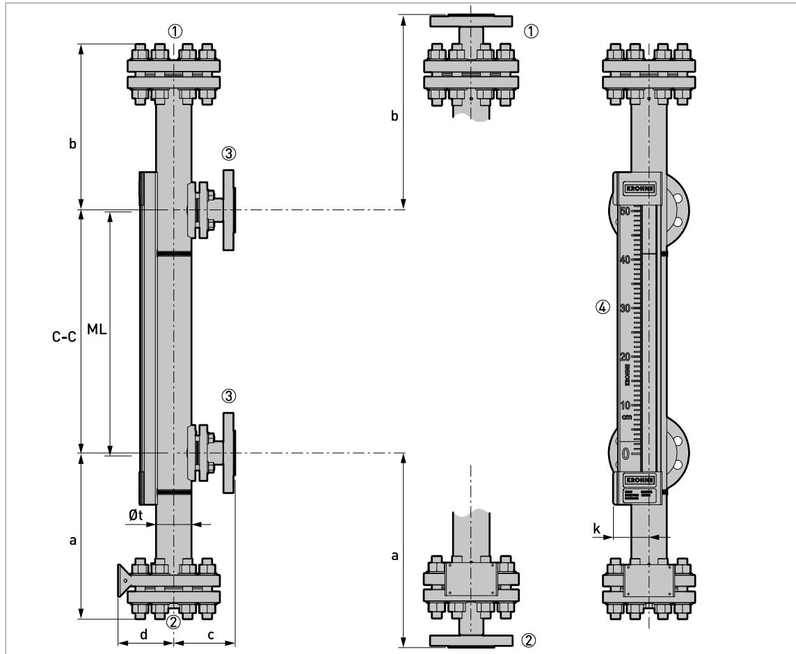
Figure 8-19: BM26A-7000 PN40 / Class 300 (PTFE-lined): side - side process connections
