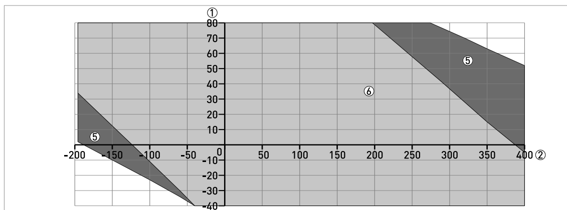
Figure 8-38: Ambient temperature / process temperature, in °C - MS15-series limit switch with the stainless-steel housing option
