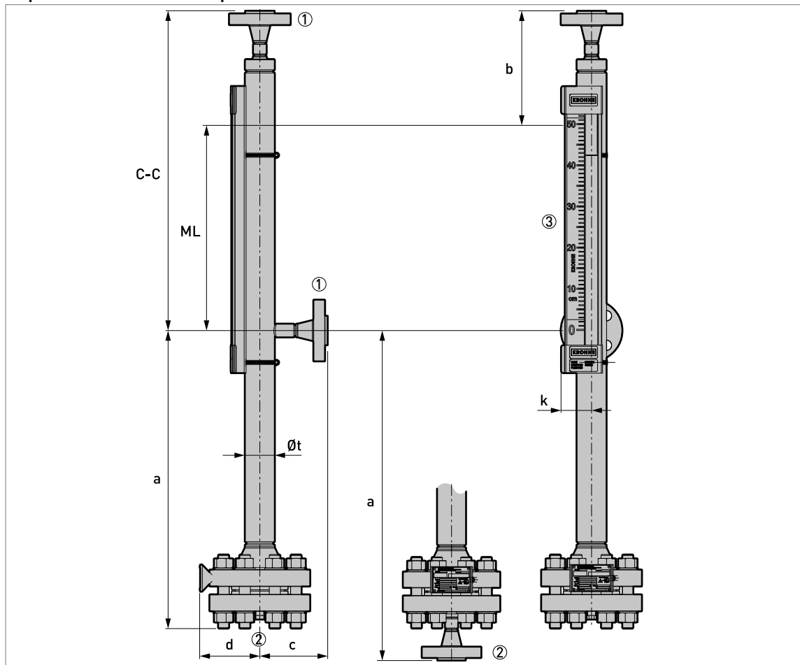
Figure 8-17: BM26A-7000 PN250 / Class 1500: top axial - bottom side process connections
