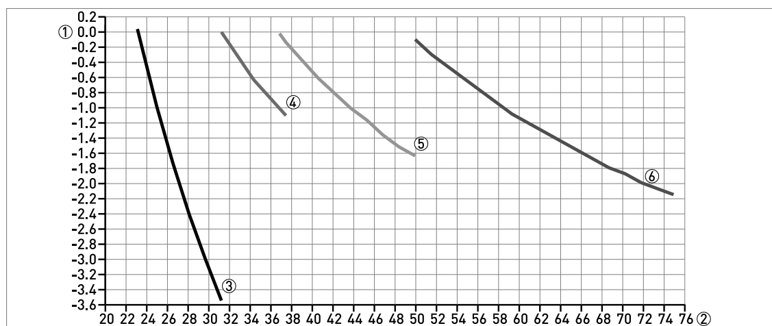
Figure 9-8: BM26A-7000 PN40 (all-metal): Float magnet offset in relation to liquid level in inches
