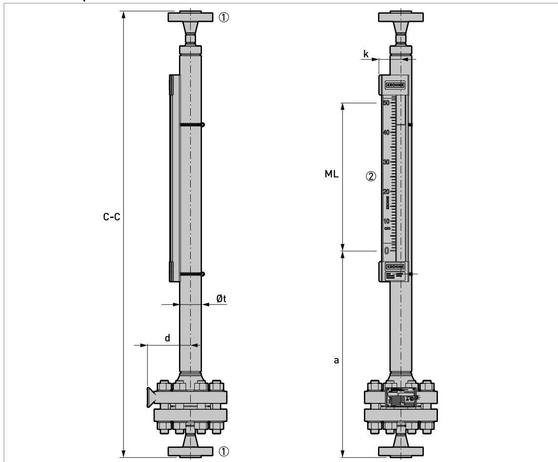
Figure 8-15: BM26A-7000 PN250 / Class 1500: axial - axial process connections
