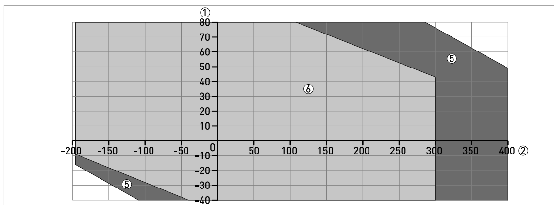
Figure 8-28: Ambient temperature / process temperature, in °C - without a thermal insulation option and without the LCD indicator module
