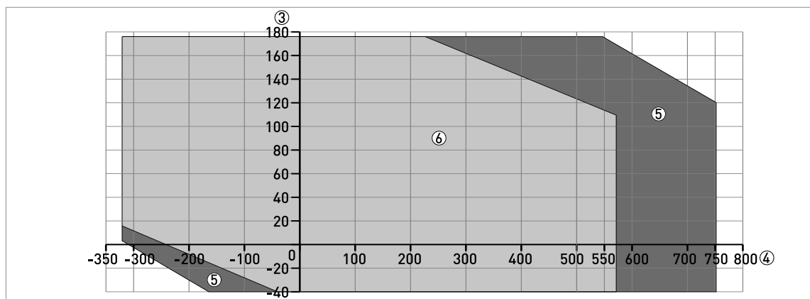
Figure 8-29: Ambient temperature / process temperature, in °F - without a thermal insulation option and without the LCD indicator module
