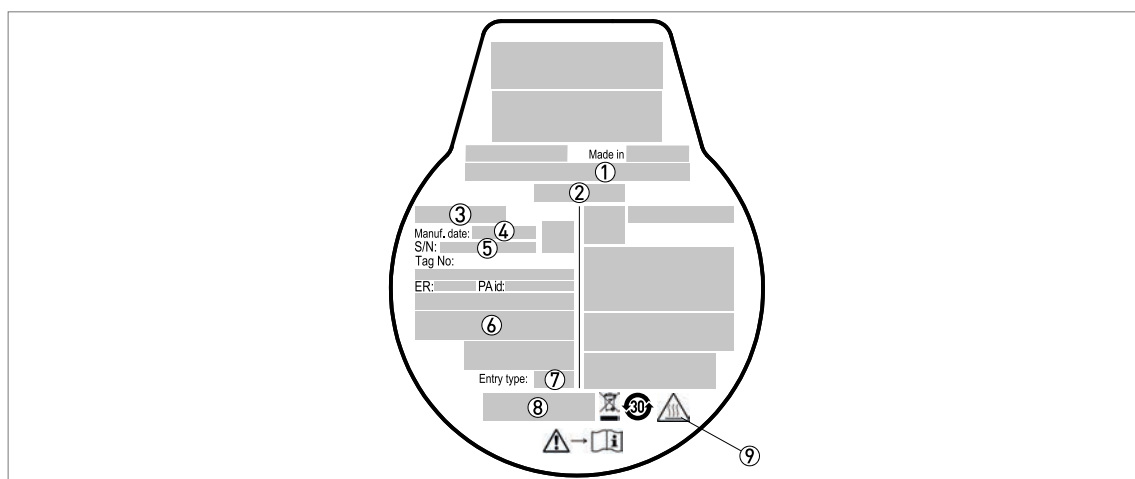
Figure 2-5: LT40 reed-chain level transmitter nameplate
