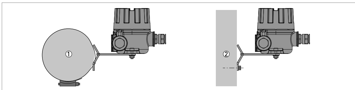
Figure 3-6: LT40 F: Installation of the remote converter - examples of locations (top view)
