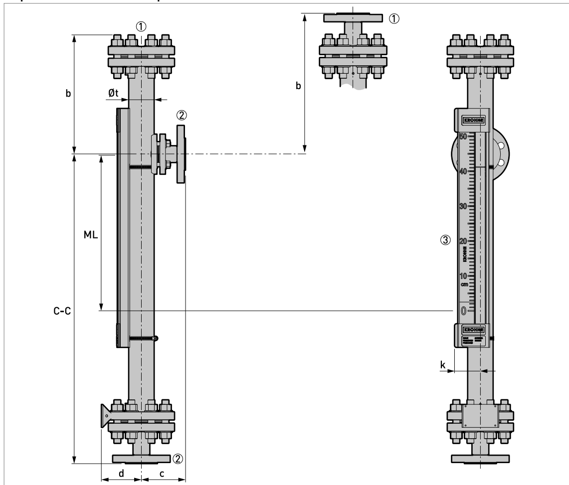
Figure 8-21: BM26A-7000 PN40 / Class 300 (PTFE-lined): top side - bottom axial process connections
