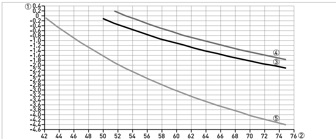
Figure 9-10: BM26A-7000 PN40 (PTFE-lined): Float magnet offset in relation to liquid level in inches
