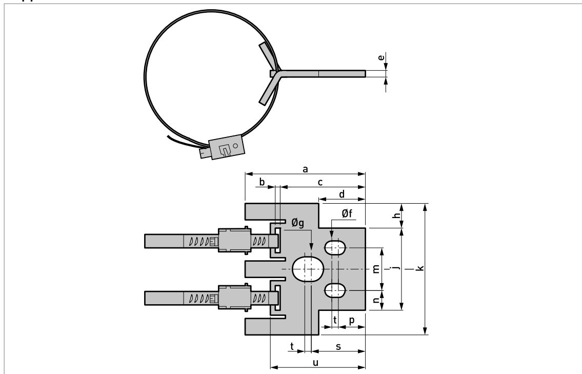
Figure 8-27: Support bracket
