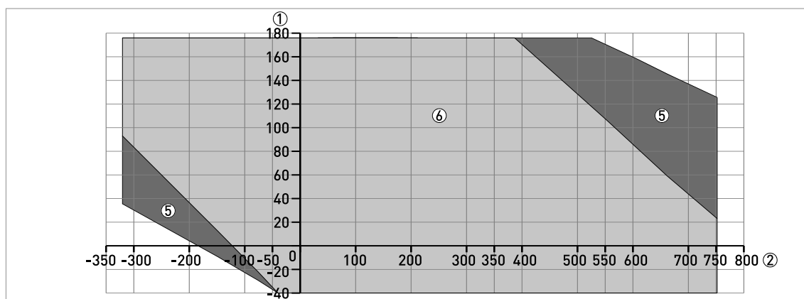
Figure 8-39: Ambient temperature / process temperature, in °F - MS15-series limit switch with the stainless-steel housing option
