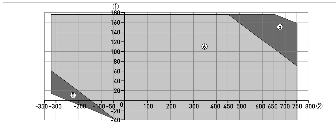
Figure 8-41: Ambient temperature / process temperature, in °F - MS40-series limit switch
