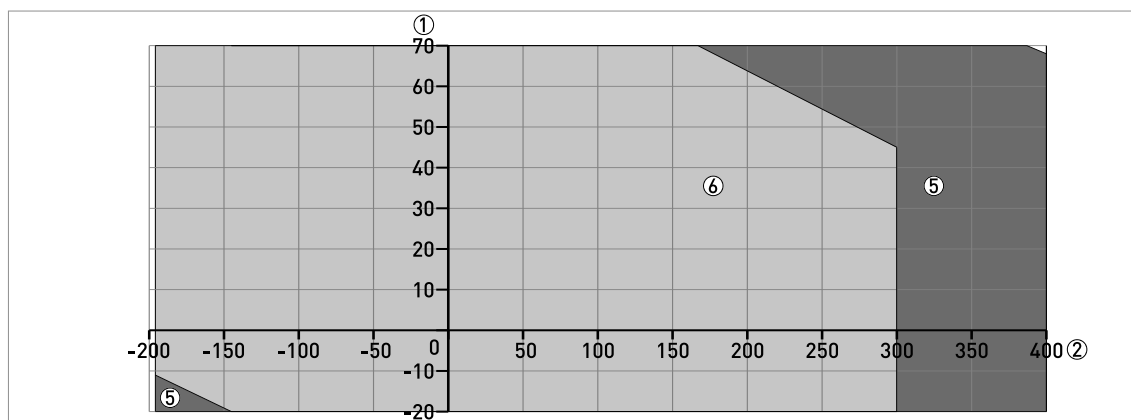
Figure 8-34: Ambient temperature / process temperature, in °C - with a thermal insulation option and with the LCD indicator module
