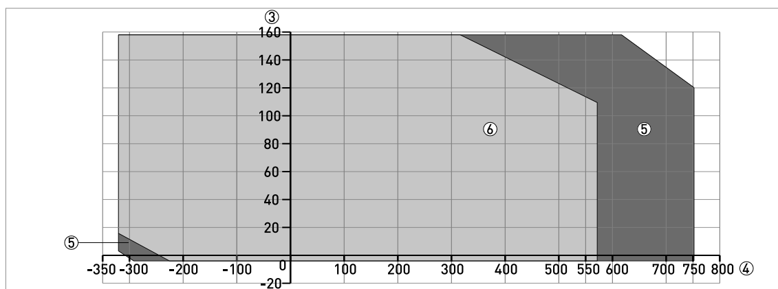
Figure 8-31: Ambient temperature / process temperature, in °F - without a thermal insulation option and with the LCD indicator module
