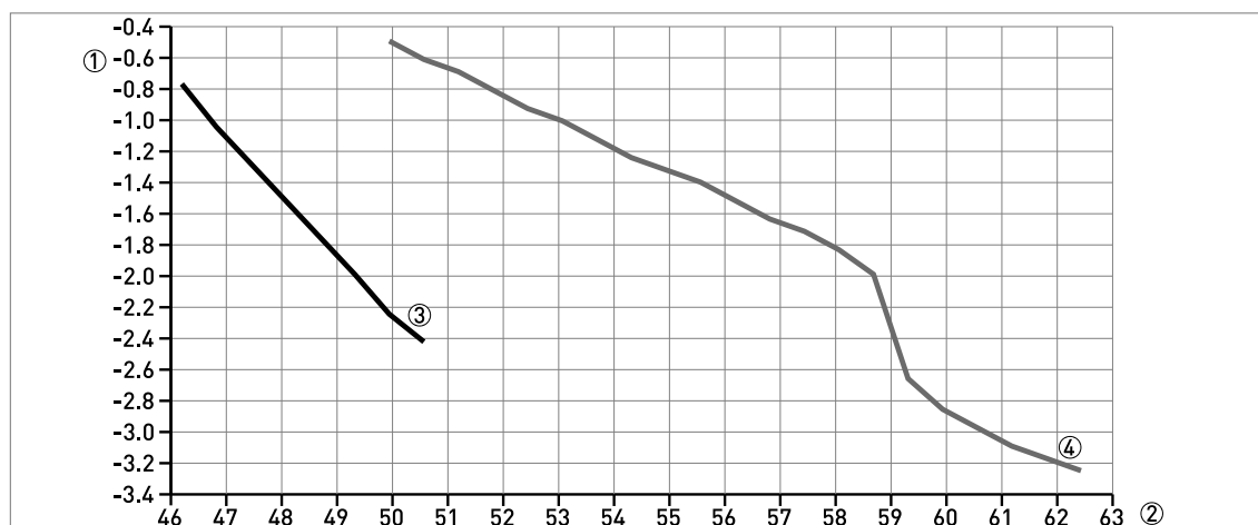
Figure 9-16: BM26A-7000 PN400: Float magnet offset in relation to liquid level in inches
