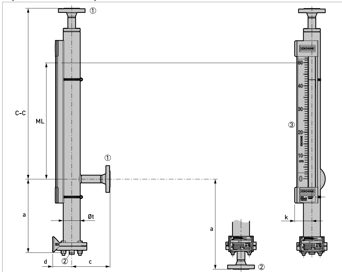
Figure 8-5: BM26A-6000: top axial - bottom side process connections
