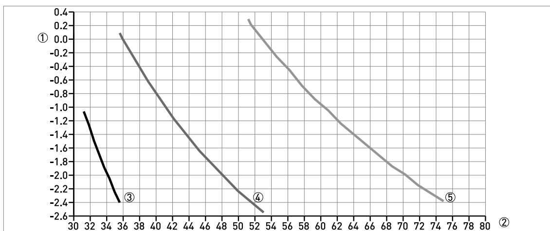
Figure 9-12: BM26A-7000 PN100: Float magnet offset in relation to liquid level in inches
