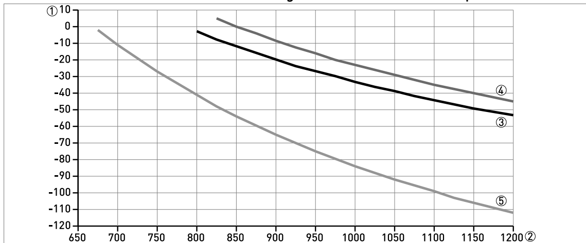
Figure 9-9: BM26A-7000 PN40 (PTFE-lined): Float magnet offset in relation to liquid level in mm
