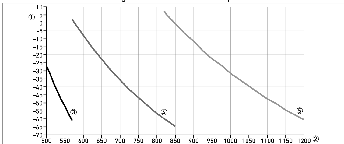
Figure 9-11: BM26A-7000 PN100: Float magnet offset in relation to liquid level in mm
