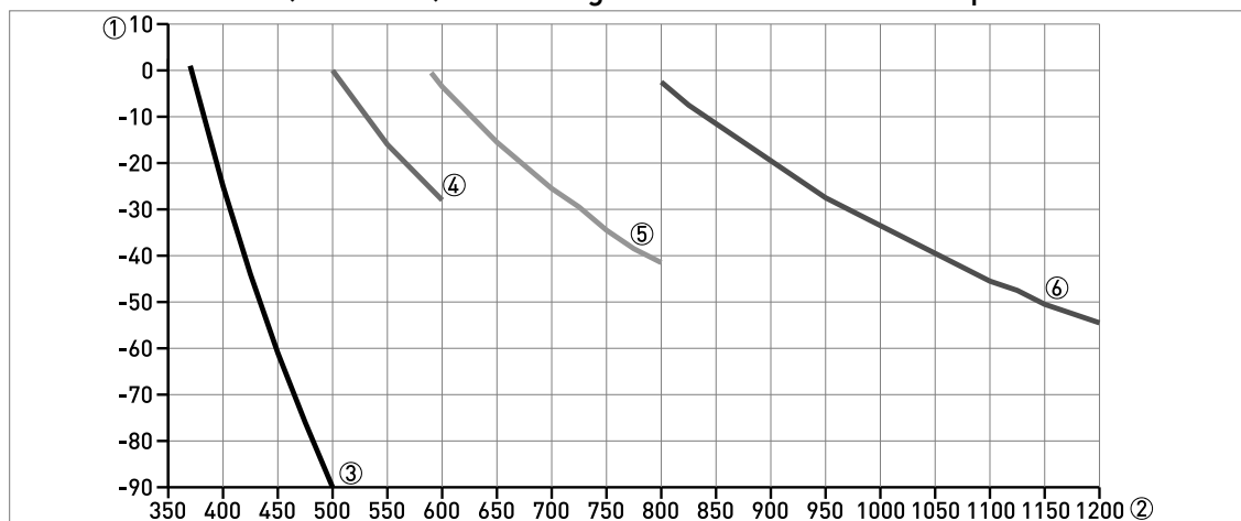
Figure 9-7: BM26A-7000 PN40 (all-metal): Float magnet offset in relation to liquid level in mm
