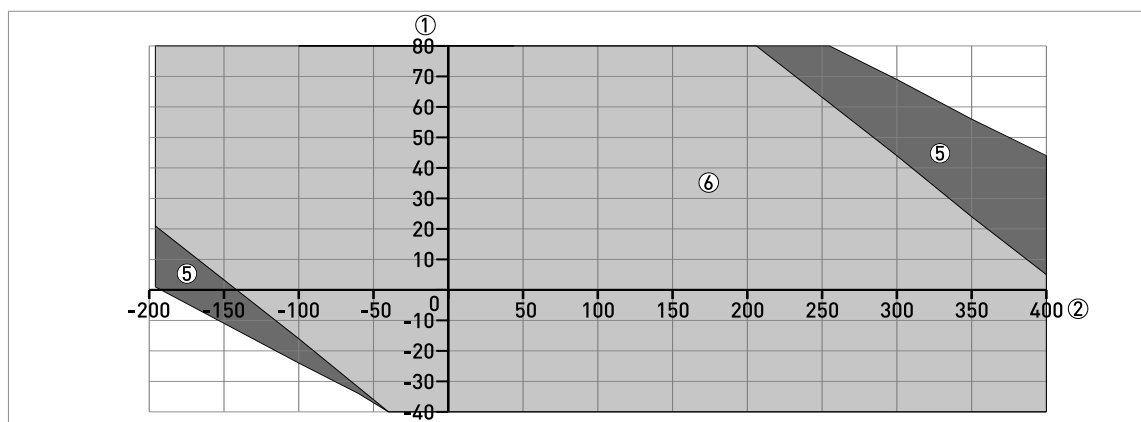
Figure 8-36: Ambient temperature / process temperature, in °C - MS15-series limit switch with the aluminium housing option
