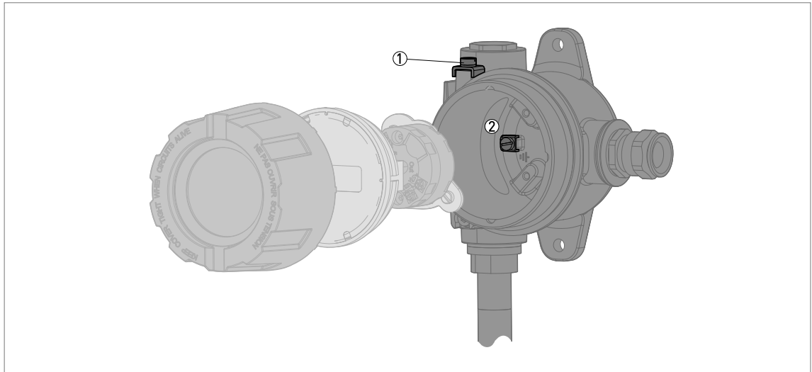
Figure 4-5: Reed-chain level transmitter - location of grounding terminals
