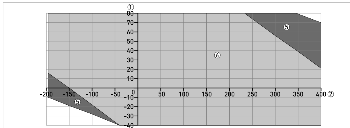
Figure 8-40: Ambient temperature / process temperature, in °C - MS40-series limit switch
