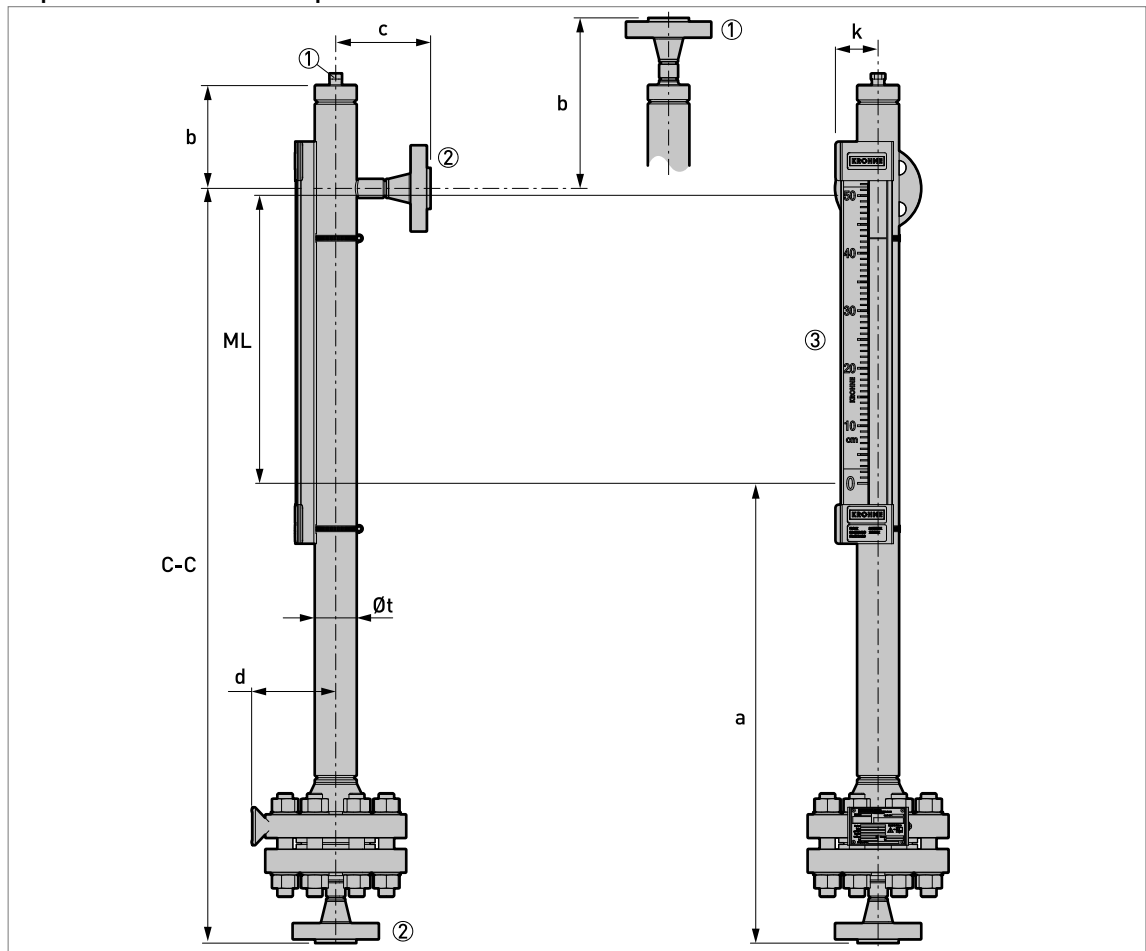
Figure 8-16: BM26A-7000 PN250 / Class 1500: top side - bottom axial process connections
