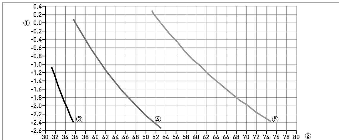
Figure 9-6: BM26A-6000: Float magnet offset in relation to liquid level in inches
