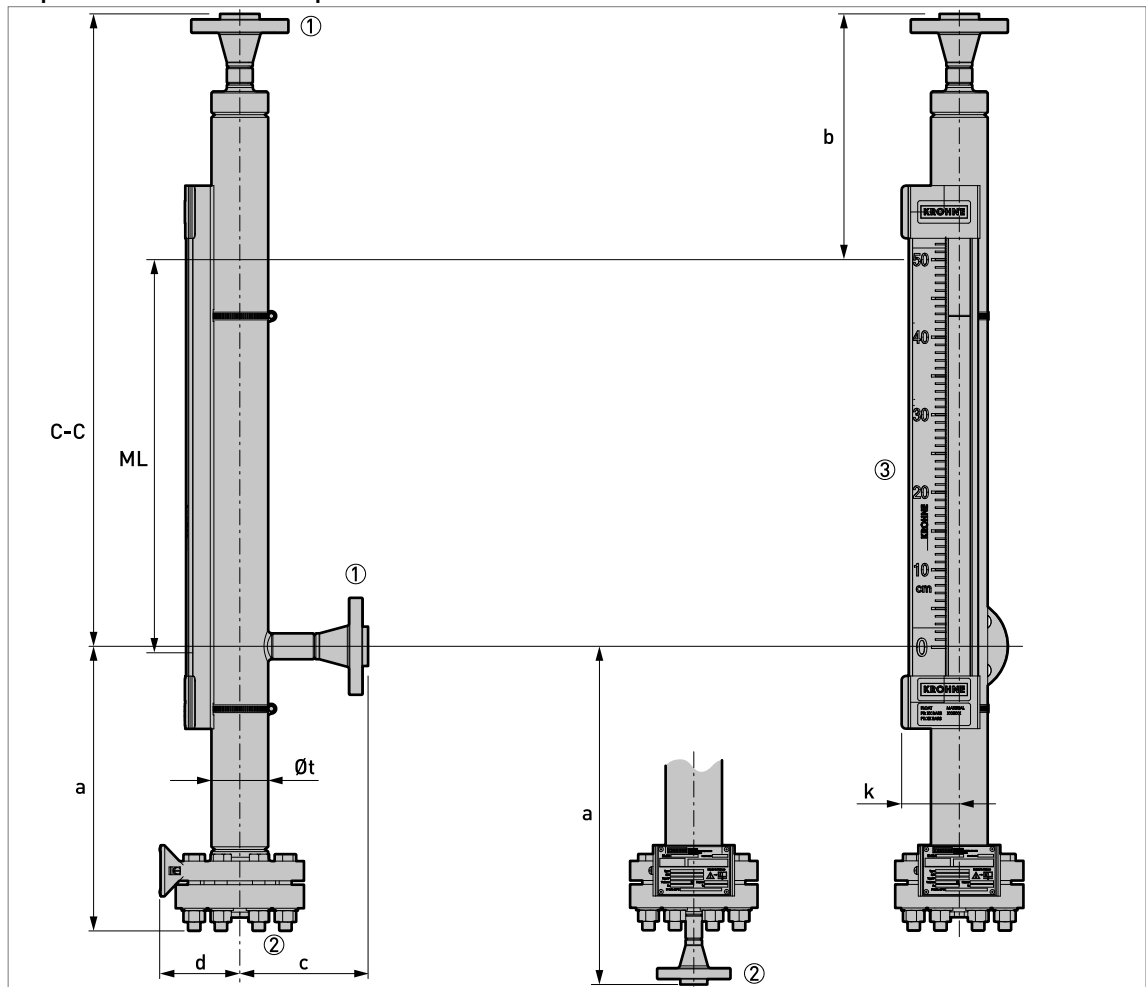
Figure 8-13: BM26A-7000 PN100 / Class 600: top axial - bottom side process connections
