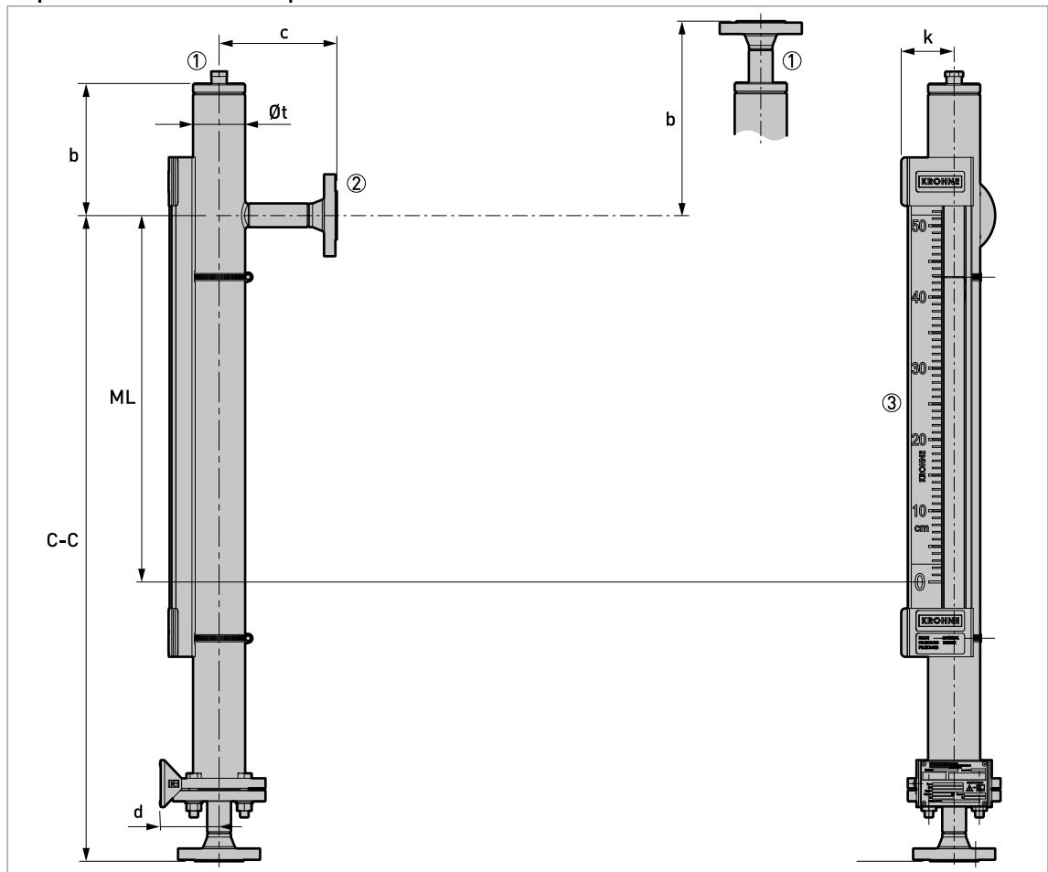
Figure 8-4: BM26A-6000: top side - bottom axial process connections
