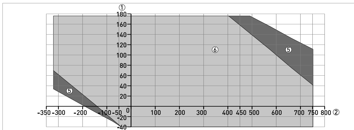
Figure 8-37: Ambient temperature / process temperature, in °F - MS15-series limit switch with the aluminium housing option
