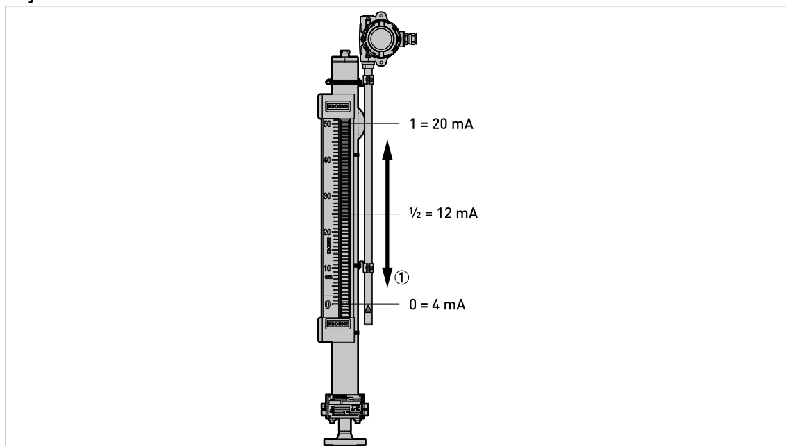
Figure 3-8: LT40: adjustments for accurate measurement of level
