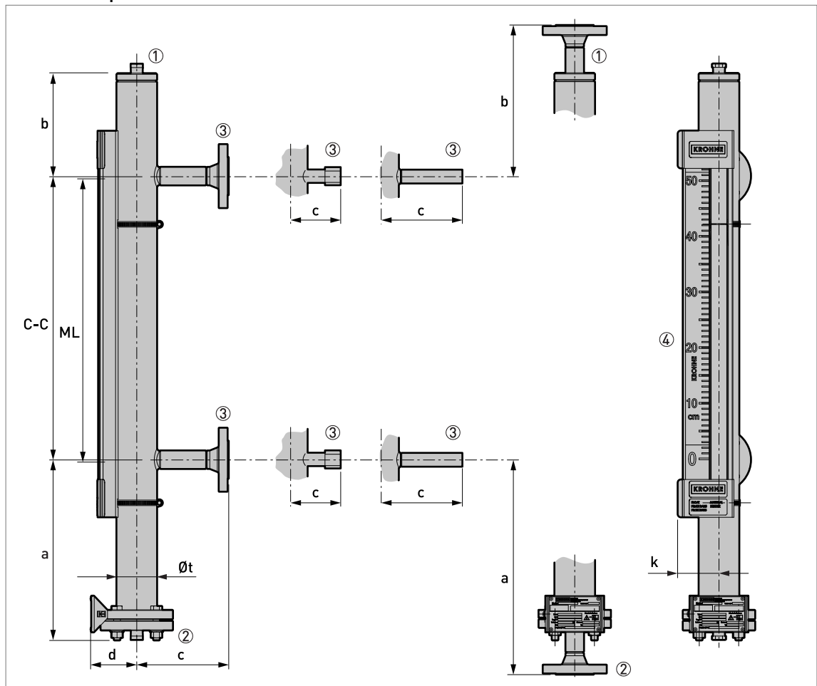
Figure 8-6: BM26A-7000 PN40 / Class 300: side - side process connections
