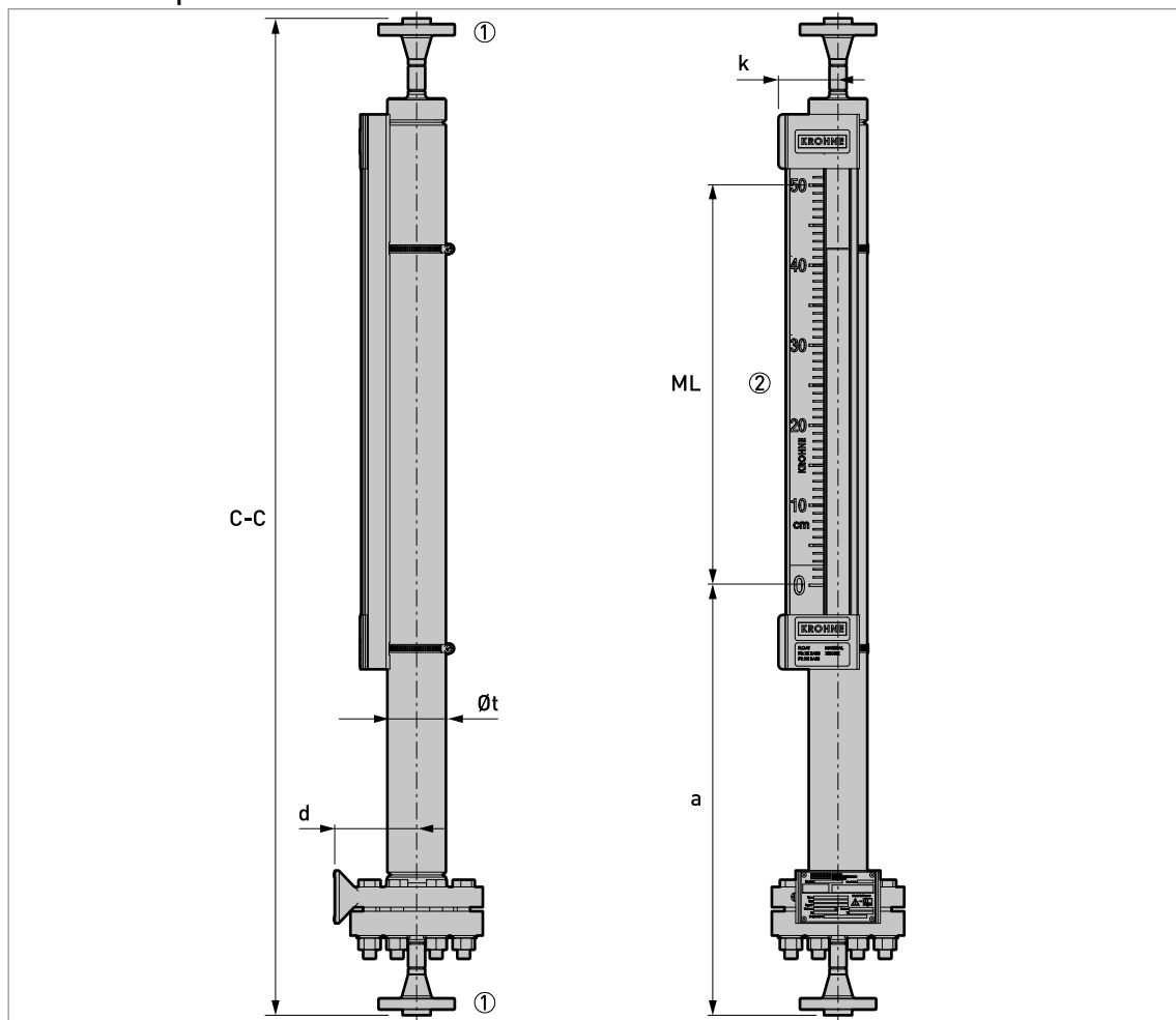
Figure 8-11: BM26A-7000 PN100 / Class 600: axial - axial process connections
