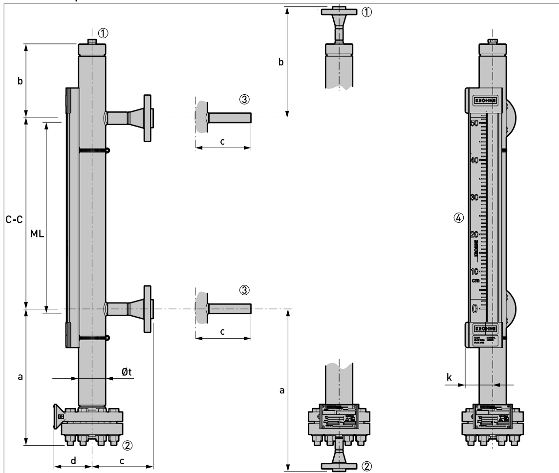
Figure 8-10: BM26A-7000 PN100 / Class 600: side - side process connections
