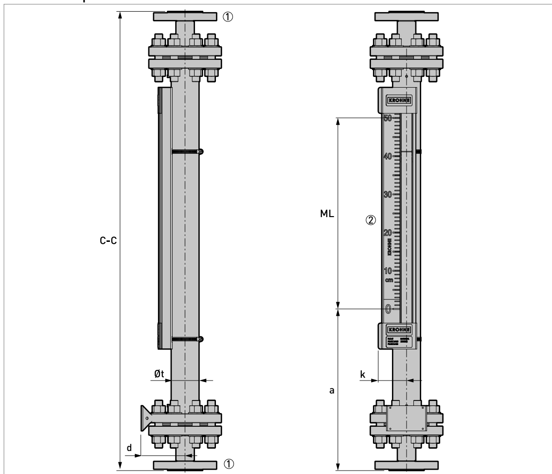
Figure 8-20: BM26A-7000 PN40 / Class 300 (PTFE-lined): axial - axial process connections
