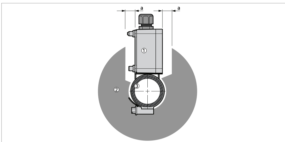
Figure 3-11: Limit switches and thermal insulation for the measuring chamber
