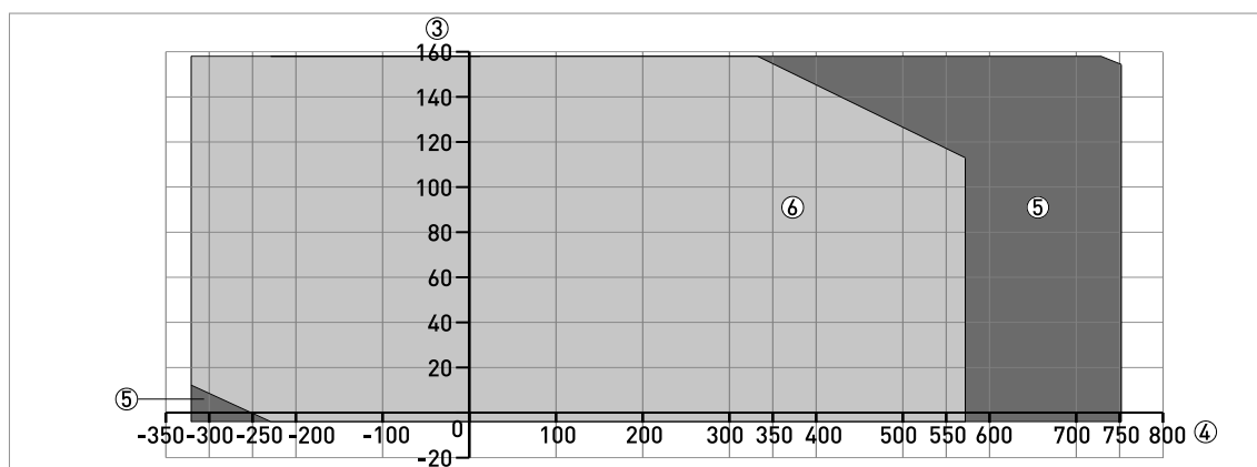
Figure 8-35: Ambient temperature / process temperature, in °F - with a thermal insulation option and with the LCD indicator module
