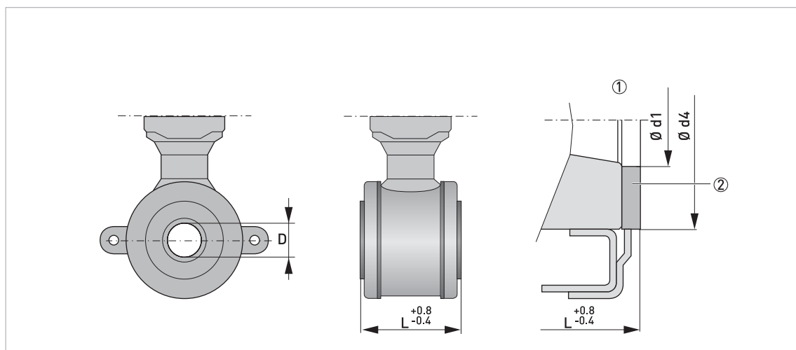
Figure 2-3: Construction details DN25...100 / 1...4"
