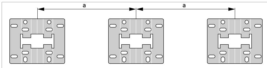
Figure 3-17: Mounting multiple devices next to each other
