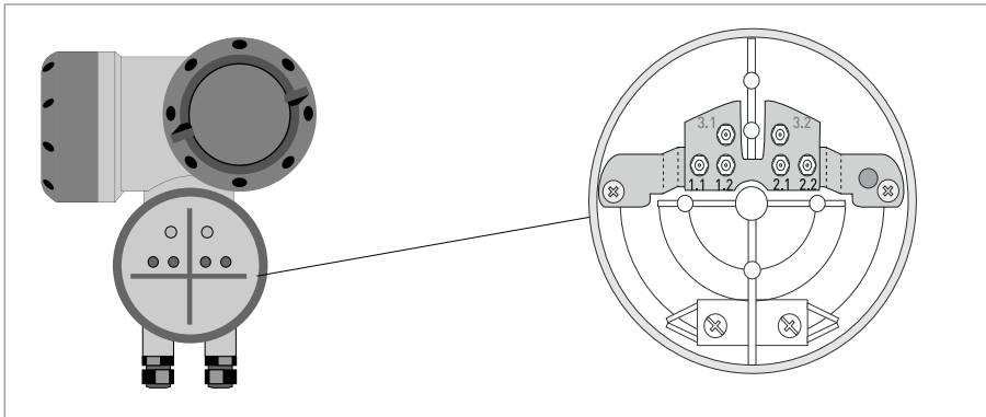
Figure 4-10: Connect signal cable
