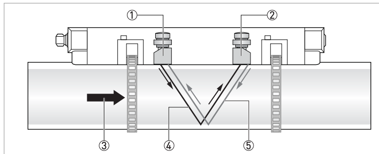
Figure 1-6: Measuring principle
