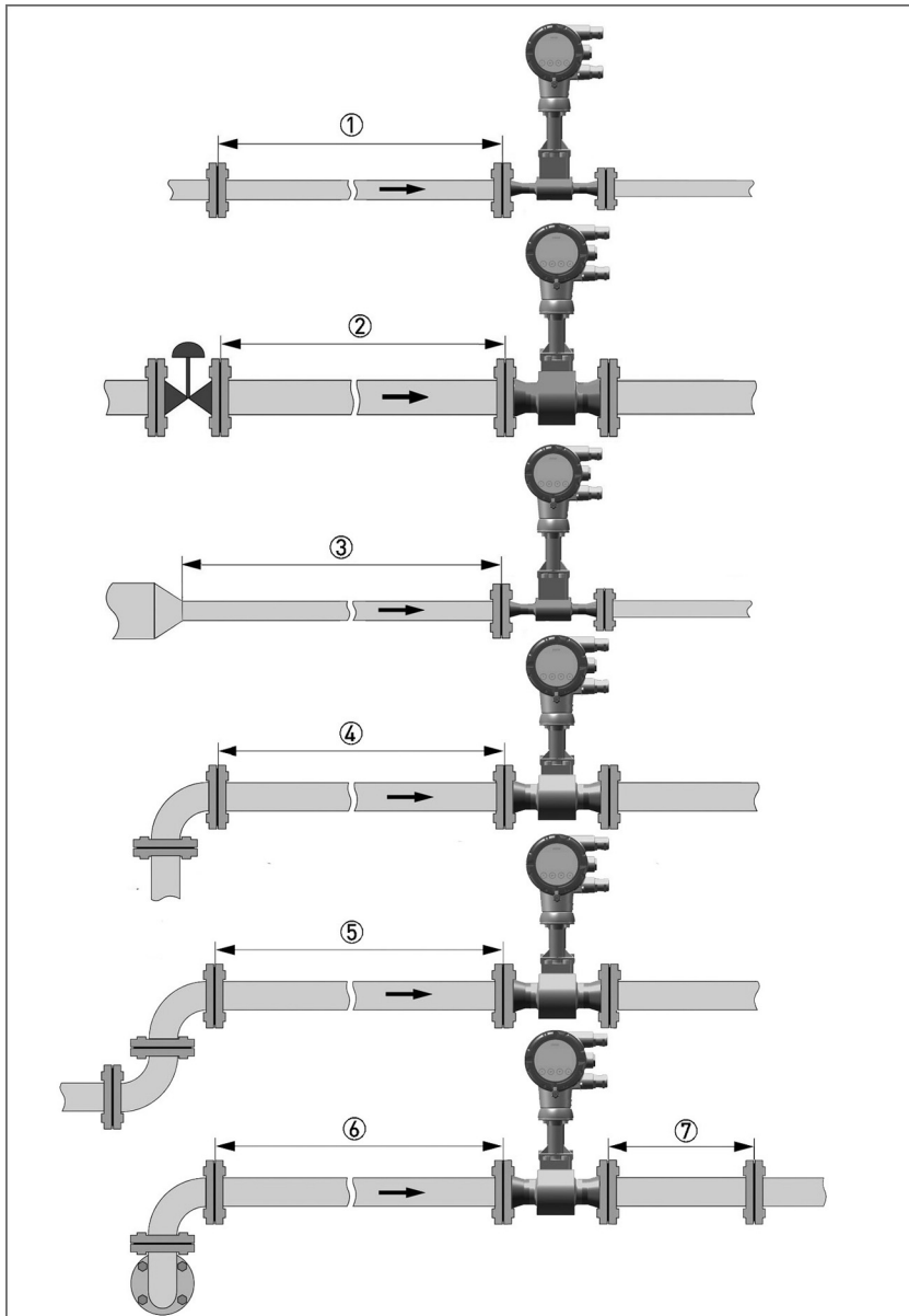
Figure 3-5: Inlet sections
