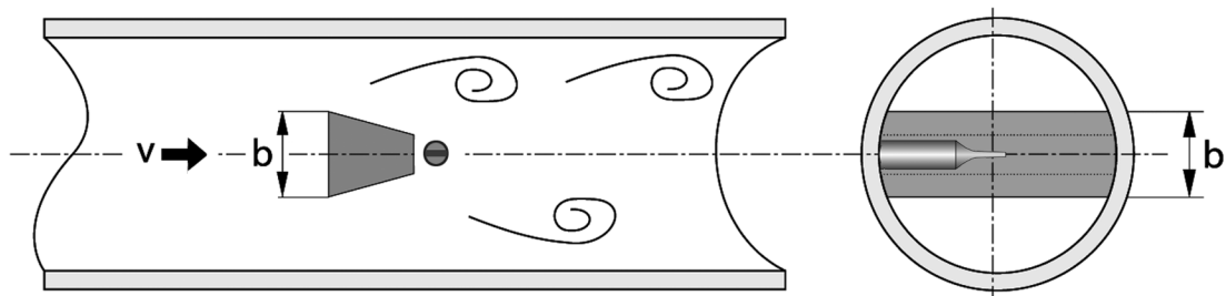
Figure 1-1: Functional principle
