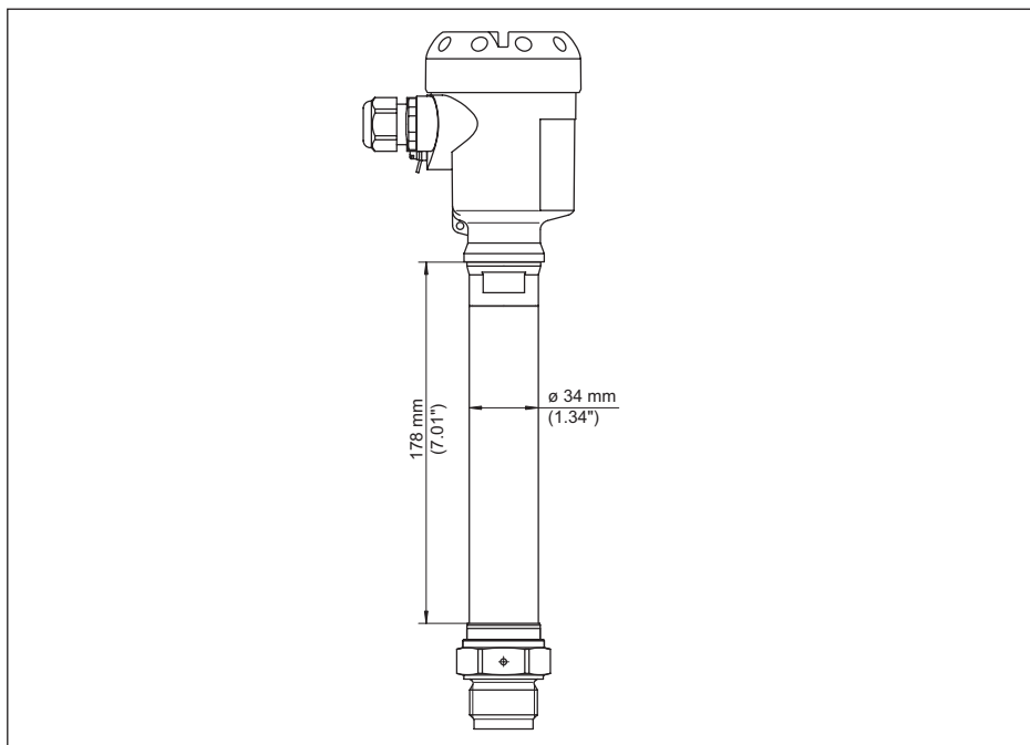
Fig. 17: Temperature adapter
