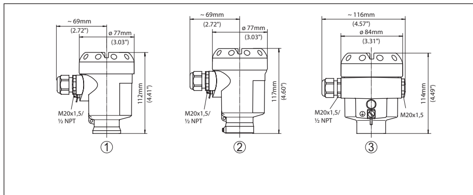
Fig. 15: Housing versions
