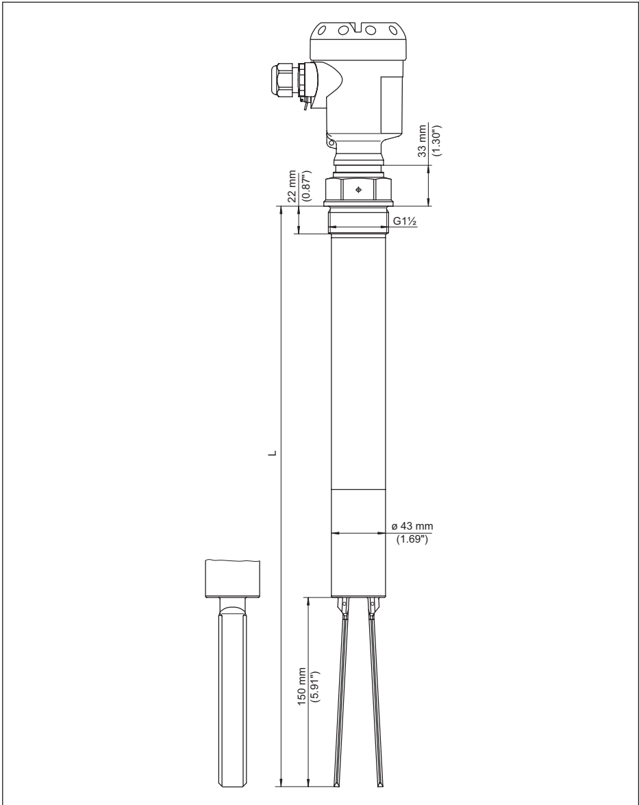
Fig. 16: OPTISWITCH 3300 C, threaded version G1 1/2 (DIN ISO 228/1)
