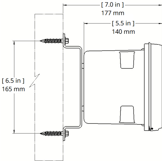
Figure 6: Wall Mount, Side View
