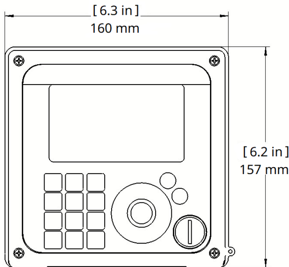
Figure 1: Panel Mount, Front View
