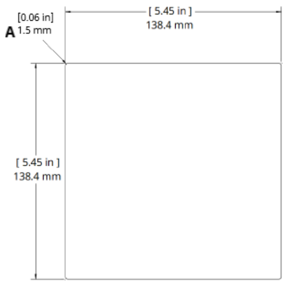
Figure 4: Panel Cut-out
