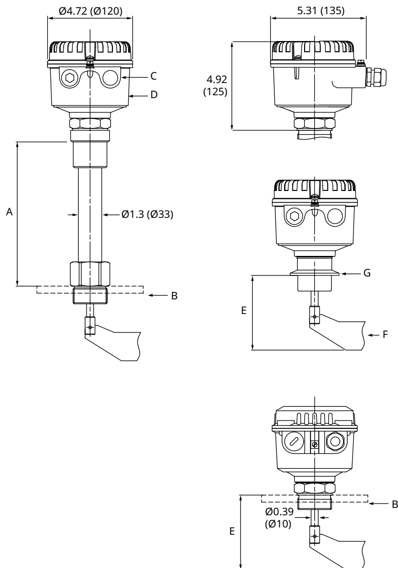
Figure 5: Rosemount 2501 Paddle Level Switch (Standard Length, Application Profile code L)
