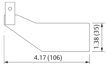
Figure 14: Boot-shaped Vane 35 x 106 mm - Code C
