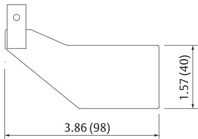
Figure 12: Boot-shaped Vane 40 x 98 mm - Code D
