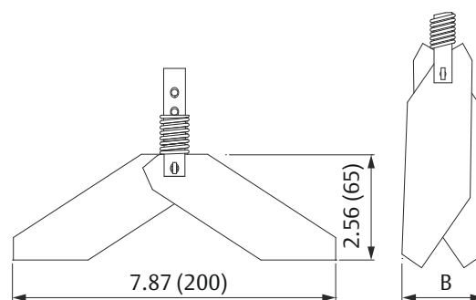
Figure 13: Hinged Vane 98 x 200 mm, Double-sided - Code V
