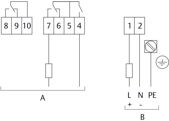
Figure 3: Terminal Block Connections for Safety Function
