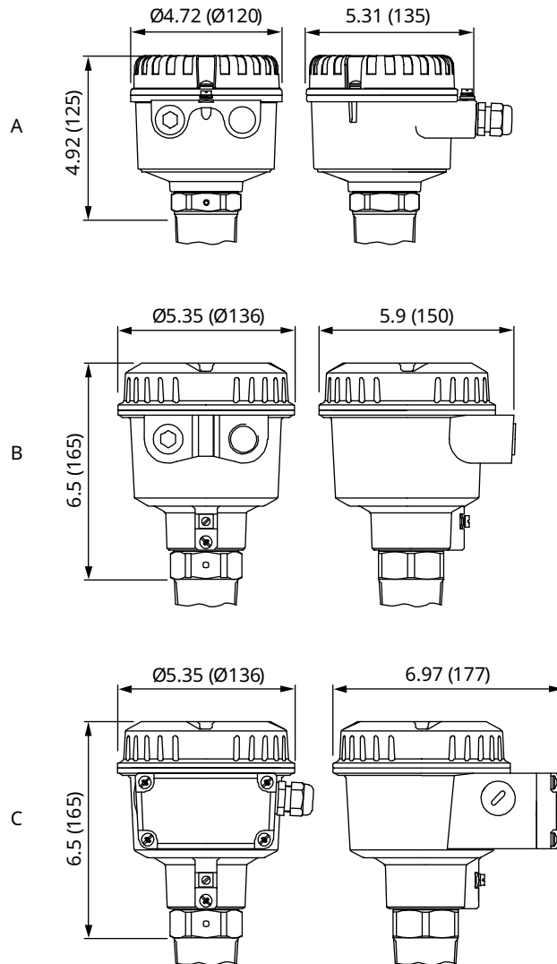
Figure 4: Rosemount 2501 Housing Options
