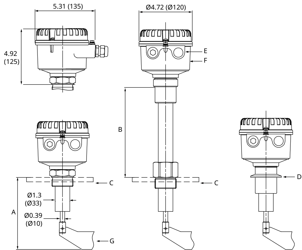
Figure 9: Rosemount 2501 Paddle Level Switch (Application Profile code J)
