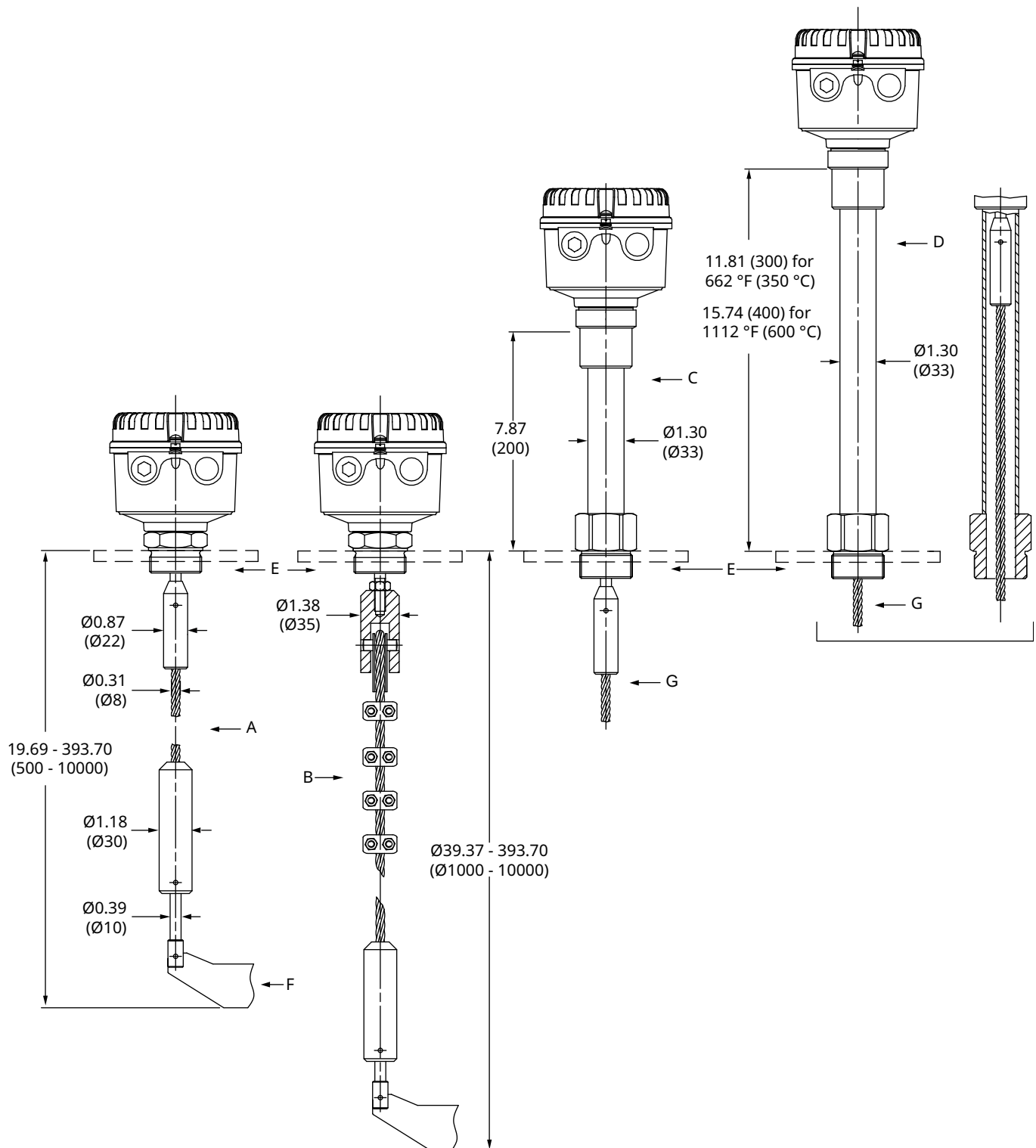
Figure 7: Rosemount 2501 Paddle Level Switch (Rope-Extended Length, Application Profile codes R and S)
