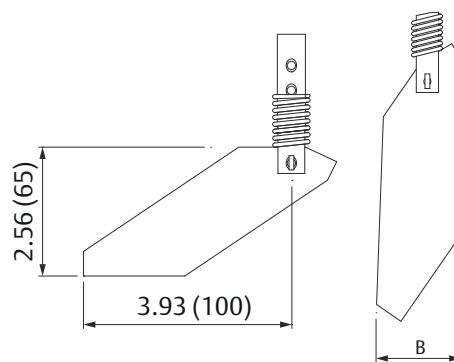
Figure 15: Boot-shaped Vane 98 x 100 mm, Single-sided - Code U
