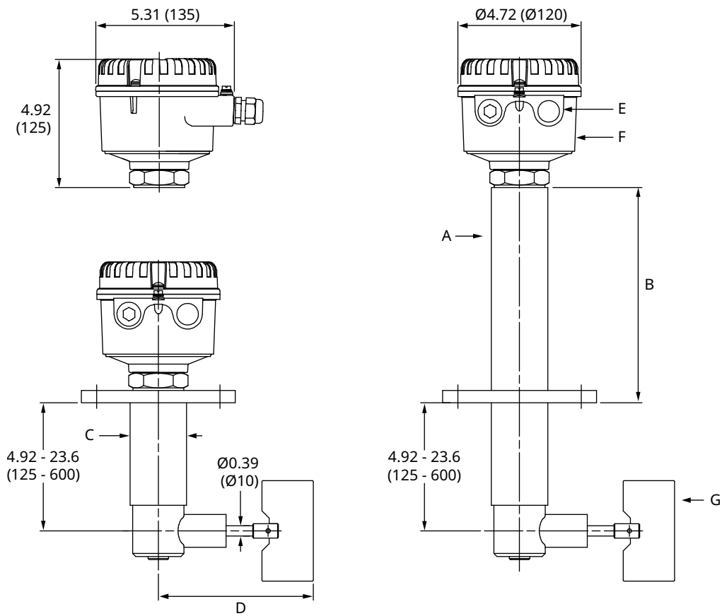
Figure 8: Rosemount 2501 Paddle Level Switch (Application Profile code K)
