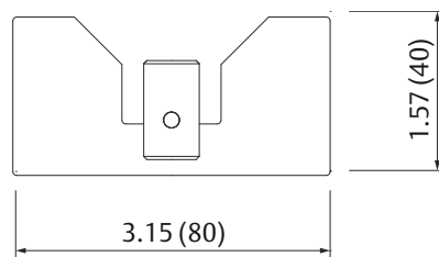
Figure 11: Rectangular Notched Vane 40 x 80 mm - Code K
