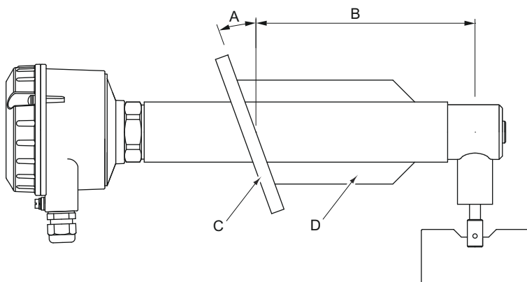
Figure 21: Process connection flange welded to paddle tube
